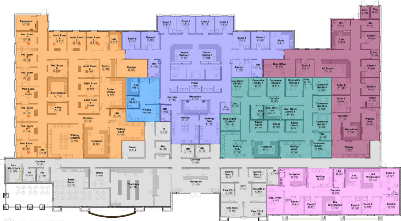
1 PRESENTATION PLAN 1/8" = 1'-0"
